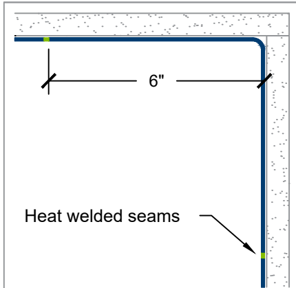
WCHW-80-IC inside corner
