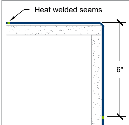
WCHW-80-OC outside corner
