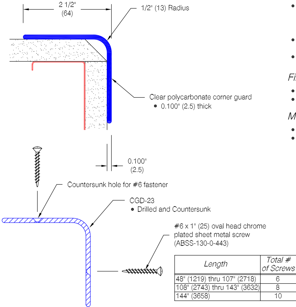
Standard Screw Mounted
