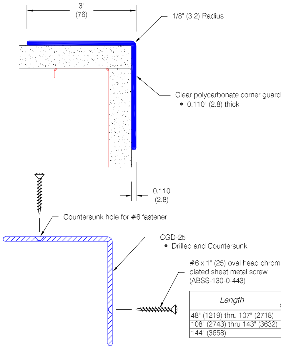
Standard Screw Mounted
