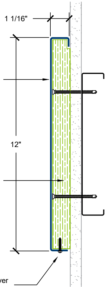
16 gauge type 304 #4 finish stainless steel cover (standard)
