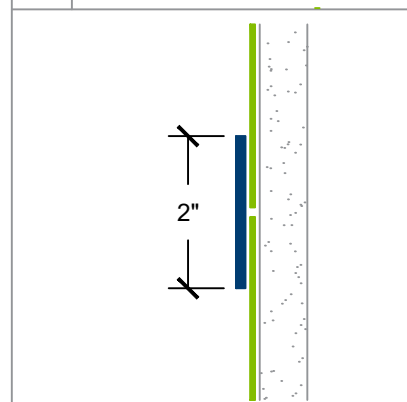
J Joint detail
