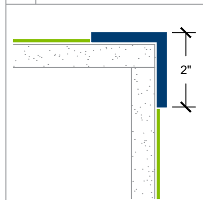
OC Outside corner detail
