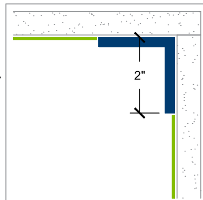
IC Inside corner detail
